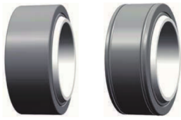
滑动摩擦副：钢 / PTFE 编织物 Sliding contact surfaces: Steel / PTFE fabric
