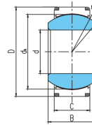
GEC(H)...XT-2RS
